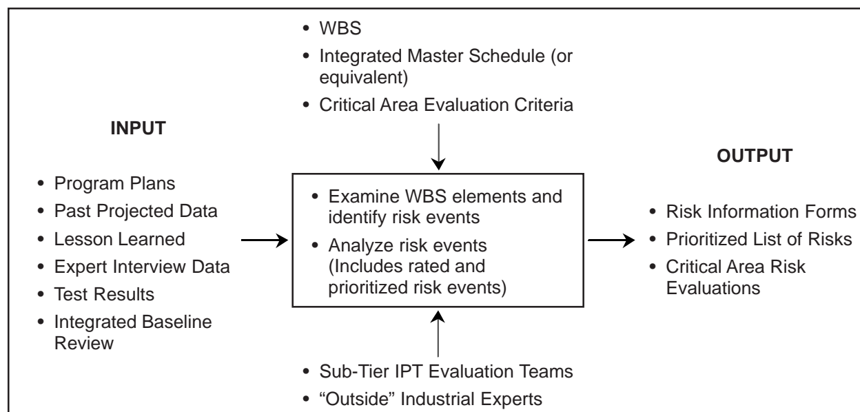
Figure 5-3. Product (WBS) Risk Assessment Technique Input and Output
